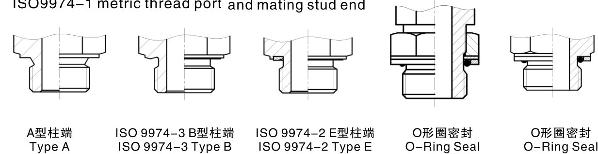
1 ISO9974-1 公制螺纹油口及相配柱端 ISO9974-1 metric thread port and mating stud end
